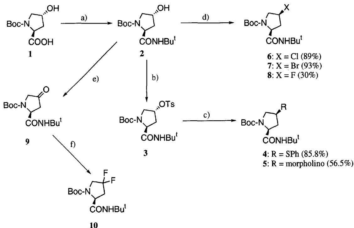
Scheme 1. Reagents and conditions: (a) isobutyl chloroformate, THF, N -methylmorpholine, t -BuNH 2 , 84.7%; (b) p -tosyl chloride, pyrrolidine, 55.8%; (c) sodium thiophenolate, DMF:AcOEt, 2:1 or morpholine; (d) CCl 4 /Ph 3 P or CBr 4 /Ph 3 P or DAST, THF; (e) oxalyl chloride/DMSO, CH 2 Cl 2 , 73.9%; (f) DAST, THF, 89%.
