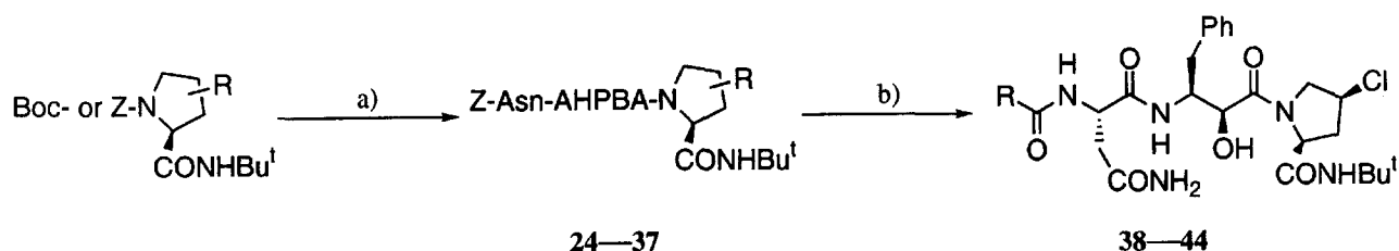
Scheme 4. Reagents and conditions: (a) (1) 4 N HCl–dioxane or \text{H}_2/10\%\text{Pd} on carbon, MeOH; (2) Z-Asn-AHPBA–OH, DEPC, \text{Et}_3\text{N} , DMF or \text{EDC} \cdot \text{HCl}/\text{HOBt} , DMF; (b) (1) \text{H}_2/10\%\text{Pd} on carbon, MeOH; (2) \text{RCOOH} , DEPC, \text{Et}_3\text{N} , DMF.
