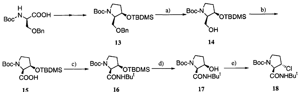
Scheme 2. Reagents and conditions: (a) Pd black, 4.4% HCOOH in MeOH, 98%; (b) Jones Reagent, acetone, 74.7%; (c) isobutyl chloroformate, THF, N -methylmorpholine, t -BuNH 2 , 47.5%; (d) ( t -Bu) 4 NF, THF; (e) CCl 4 /Ph 3 P, THF.
