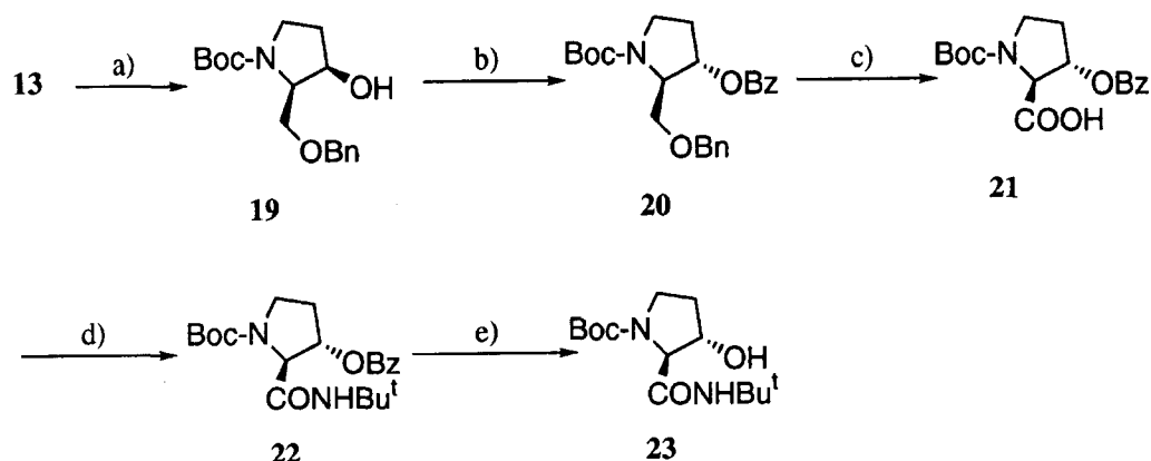
Scheme 3. Reagents and conditions: (a) (t\text{-Bu})_4\text{NF} , THF, 99%; (b) diethyl azodicarboxylate, \text{Ph}_3\text{P} , THF, 78.5%; (c) (1) Pd black, 4.4% \text{HCOOH} in MeOH; (2) Jones Reagent, acetone; (d) isobutyl chloroformate, N -methylmorpholine, THF, \text{BuNH}_3 ; (e) 1 N NaOH, MeOH, 78.5%.
